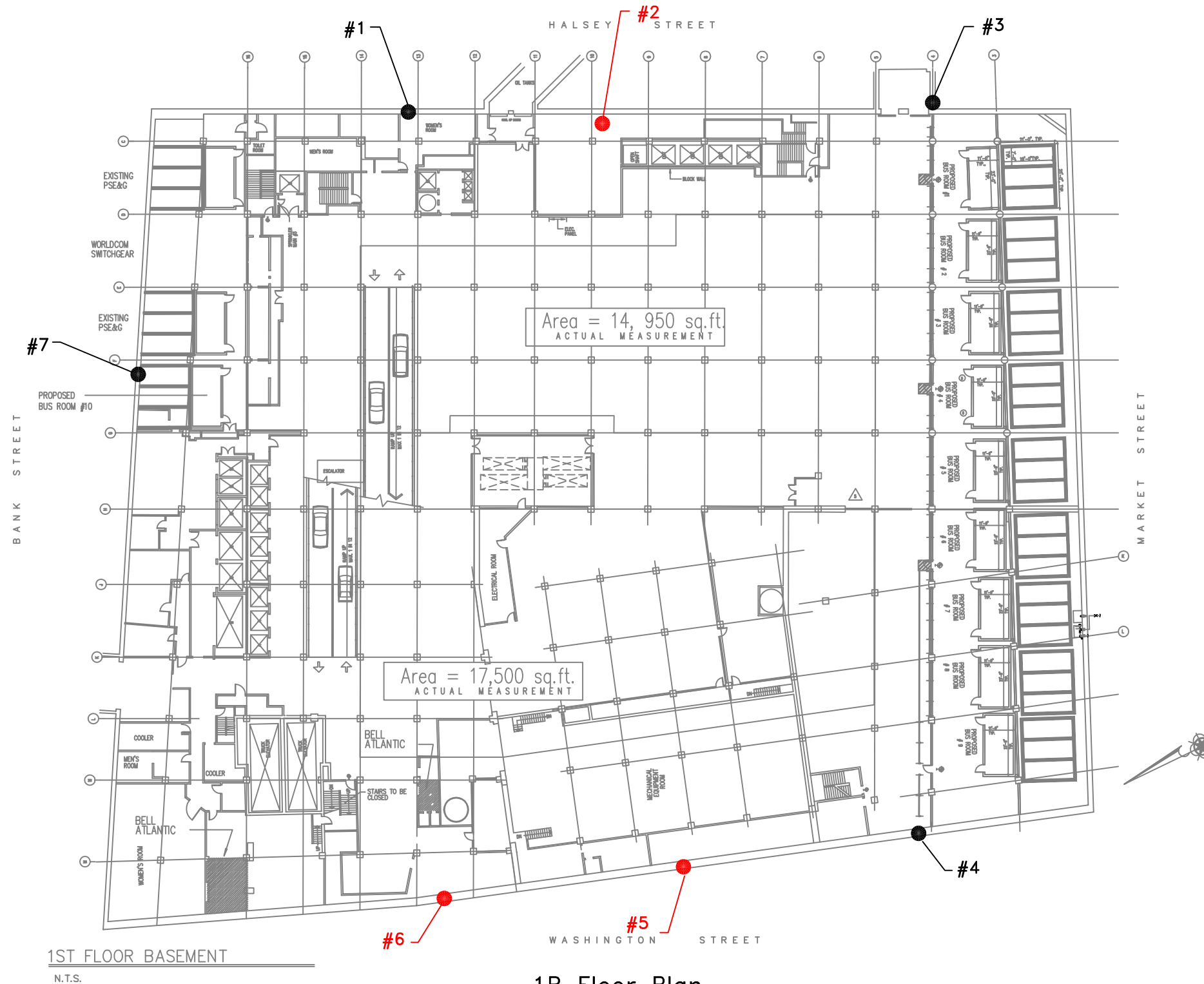
1B Floor Plan Point of Entry
